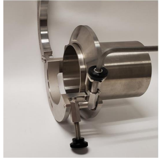
Pictured: Tack Clamp open with allen wrench for precision alignment.
